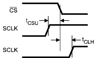
SCLK and CS Timing Parameters
